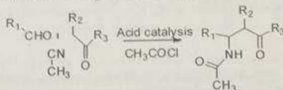
Scheme 1. Acid catalyzed stereoselective multi-component synthesis of \beta -acetamido ketones.
